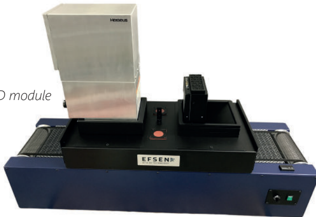
LT6-3boot with F300, 160 W/cm Arc & LED module
